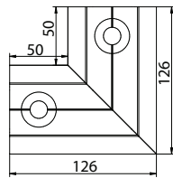
BV8900 Corner 90° (Universal) Anodized aluminium. Code: C8900
