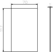
END COVER Anodized aluminium Code: BV8901K
