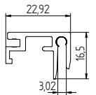
3mm BOND TRIM Anodized aluminium Code: BV9900X3
