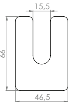
SHIMS STAINLESS STEEL Code: SH8900 (thickness upon request)
