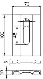
DRAINAGE PLATE Anodized aluminium Code: BV8900DP/5, BV8900DP/10
