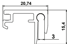
3mm BOND TRIM Eloxiertes Aluminium Code: BV7600X3
