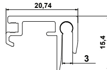
3mm BOND TRIM Eloxiertes Aluminium Code: BV7600X3
